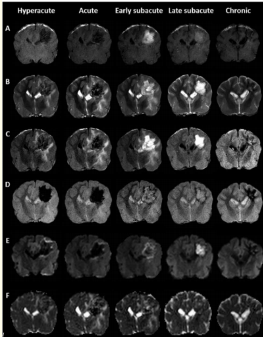
Figure 1: Representative (A) T1WI, (B) T2WI, (C) FLAIR, (D) GRE, (E) DWI, and (F) ADC maps illustrating the temporal evolution of hemorrhagic lesions according to the evolving stages. Hematomas in the right side of the parietal lobe underwent rapid and reversible changes in signal intensity, which varied with the pulse sequence. From: Daegi An., et al [8]. There is a persistent black out effect noted in ADC map images.
