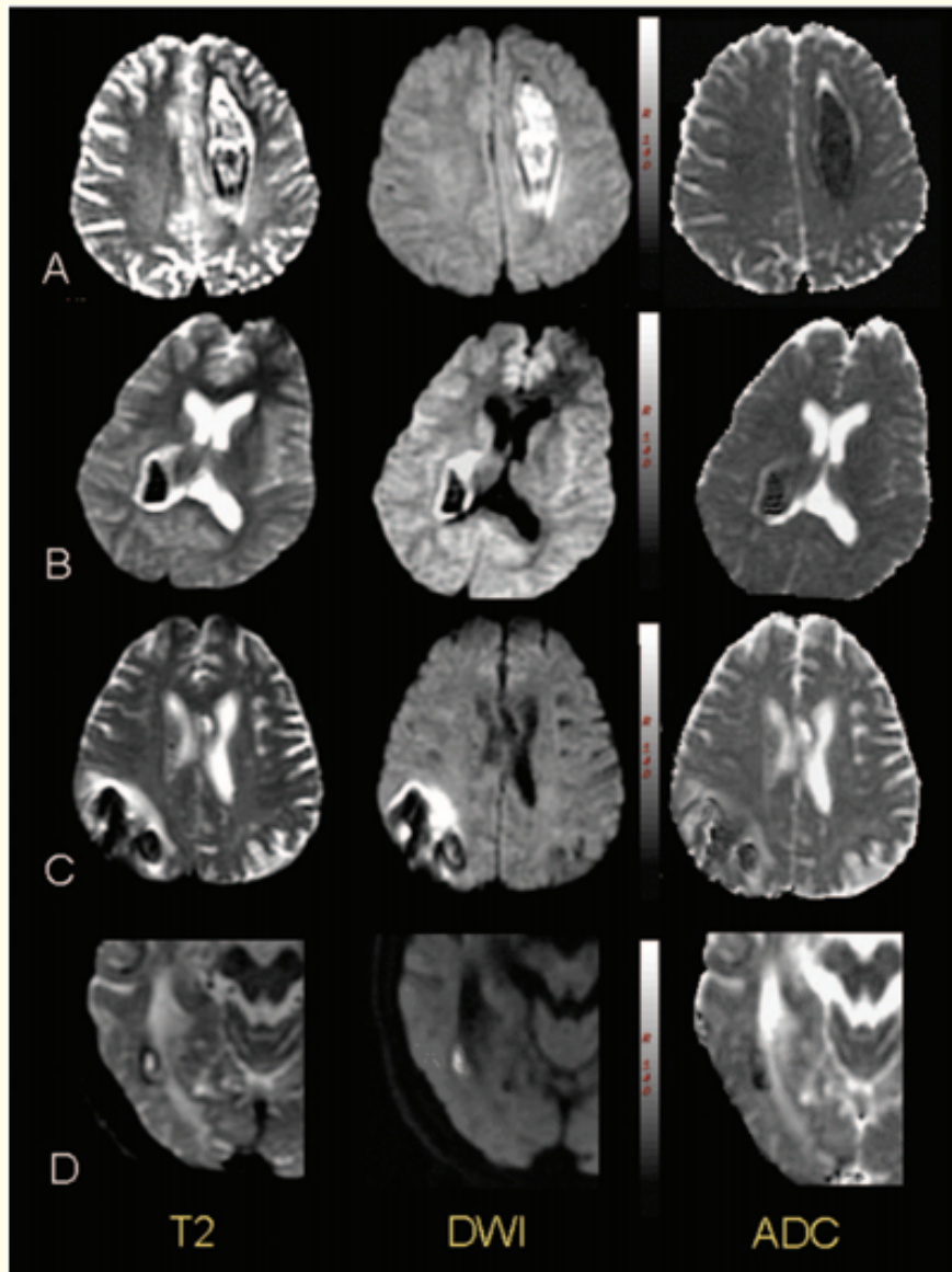
Figure 2: T2 shine-through (A, D) and T2 blackout effects (B, C) in intracerebral hematomas. A, Hyperacute hematoma in a 28-year-old man. The frontal lobe hematoma is isointense on a T1-weighted, hyperintense on a fluid-attenuated inversion recovery (not shown), T2-weighted, and DW image acquired with low ADC values. B, Acute hematoma in a 19-year-old woman. The right capsule-thalamic hematoma is isointense on a T1-weighted (not shown), hypointense on a T2-weighted, and hypointense on a DW image with low ADC values. C, Early subacute hematoma in a 54-year-old man. The right parietal lobe hematoma is hyperintense on a T1-weighted (not shown), hypointense on a T2-weighted, and hypointense on a DW image acquired with low ADC values. D, Late subacute hematoma in a 73-year-old man. The right temporo-occipital hematoma is hyperintense on a T1-weighted (not shown), hyperintense on a T2-weighted, and hyperintense on a DW image acquired with low ADC values. From: Stephane Silvera., et al [9]. There is a persistent black out effect noted in ADC map images.
